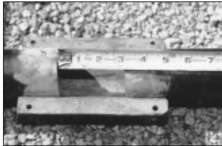
Fig. 10. Damaged areas up to 3 inches in length can be repaired simply by removing the affected pipe and enclosing the gap with a coupling.
